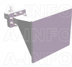
LB-137-15-C-TFSPO Standard Gain Horn Antenna 5.85-8.2GHz 15dB Gain TNC Female
